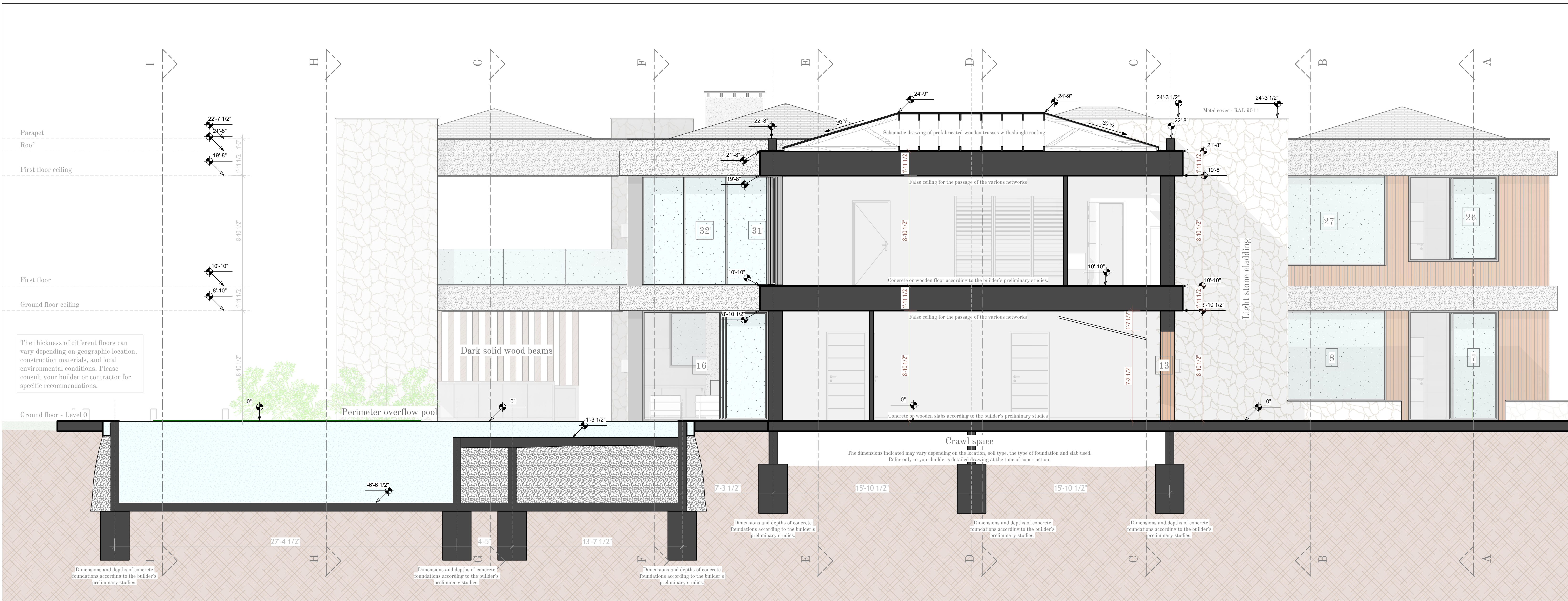
Section M-M
