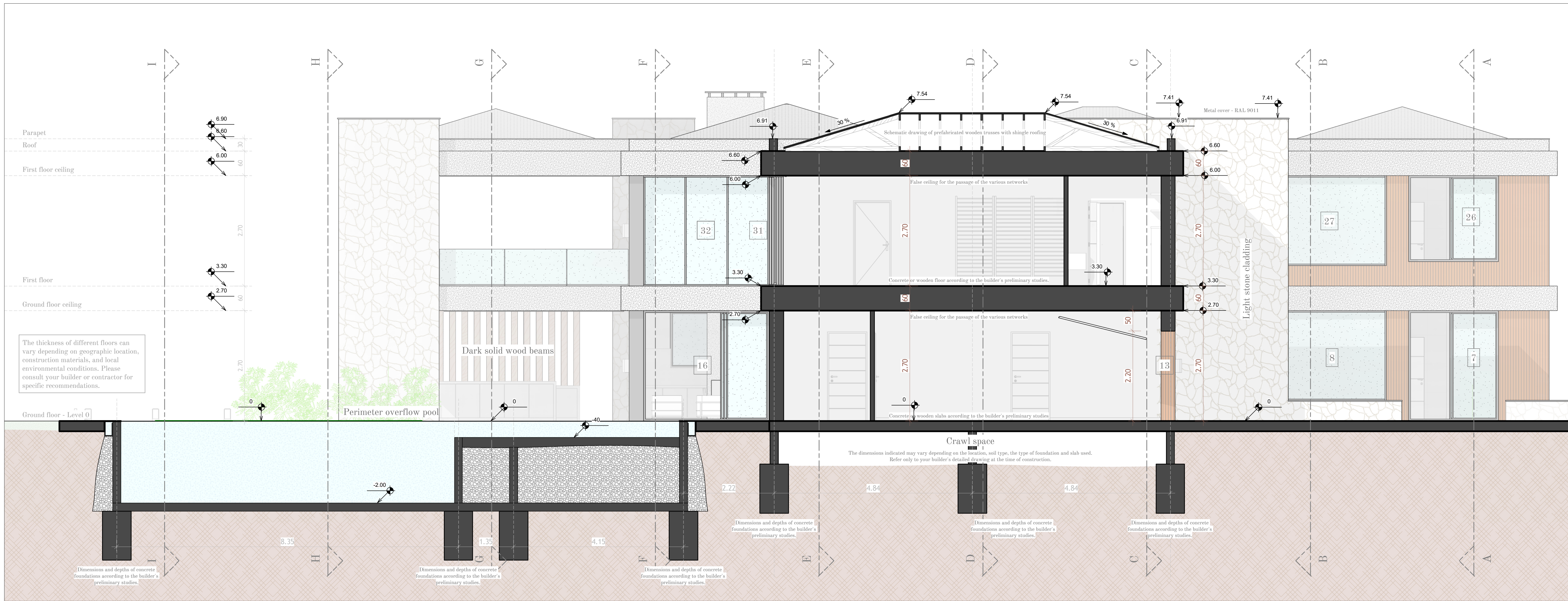
Section M-M
