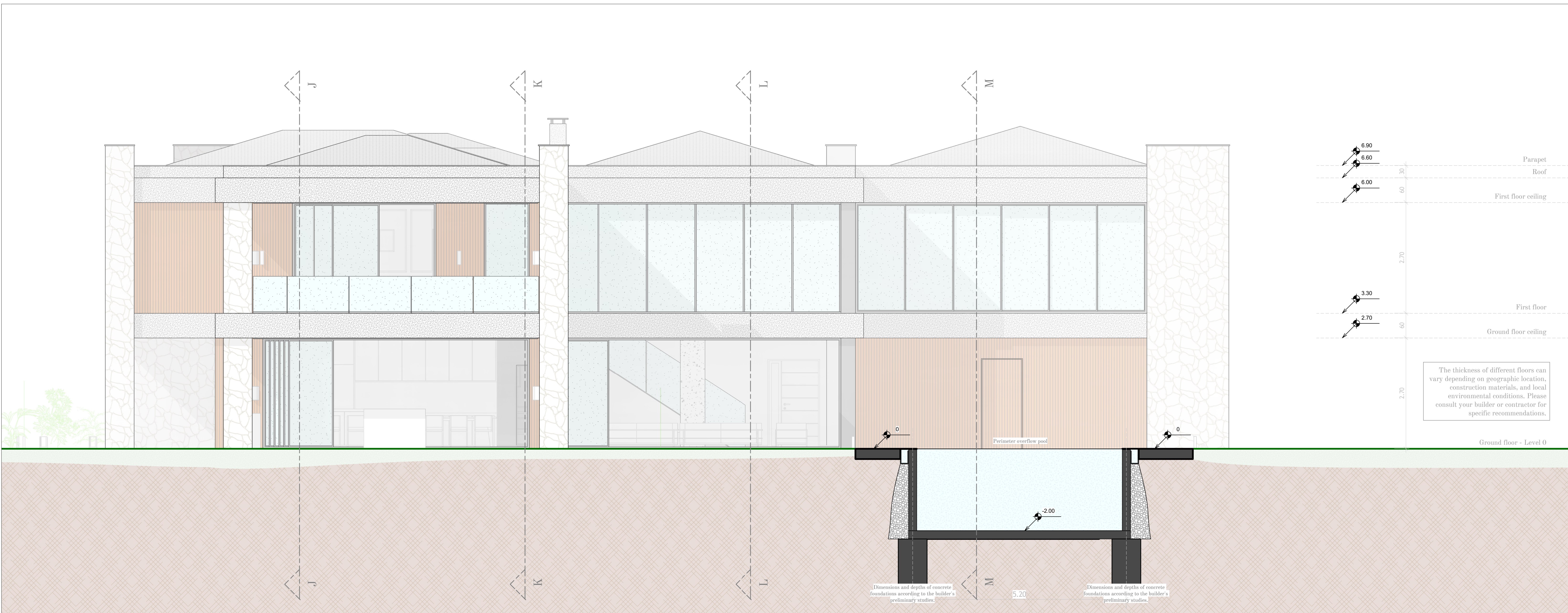
Section I-I
