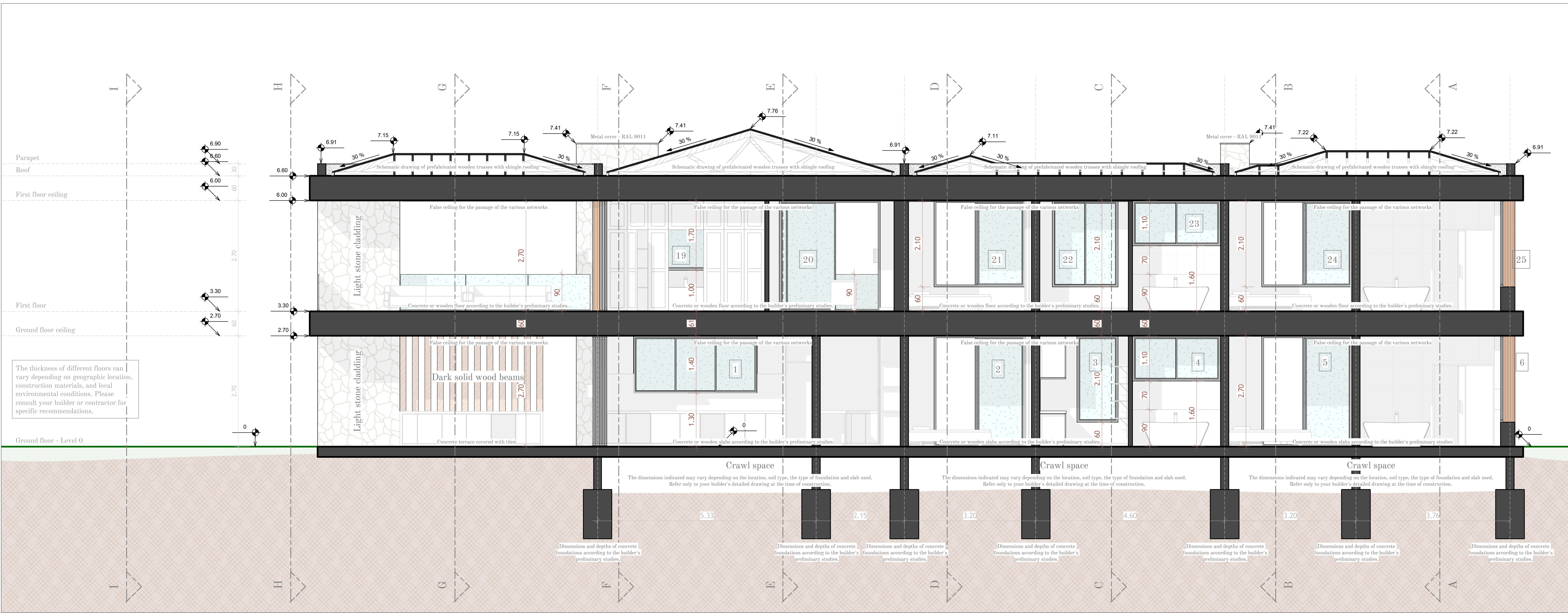
Section J-J
